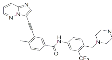
Chemical Structure
